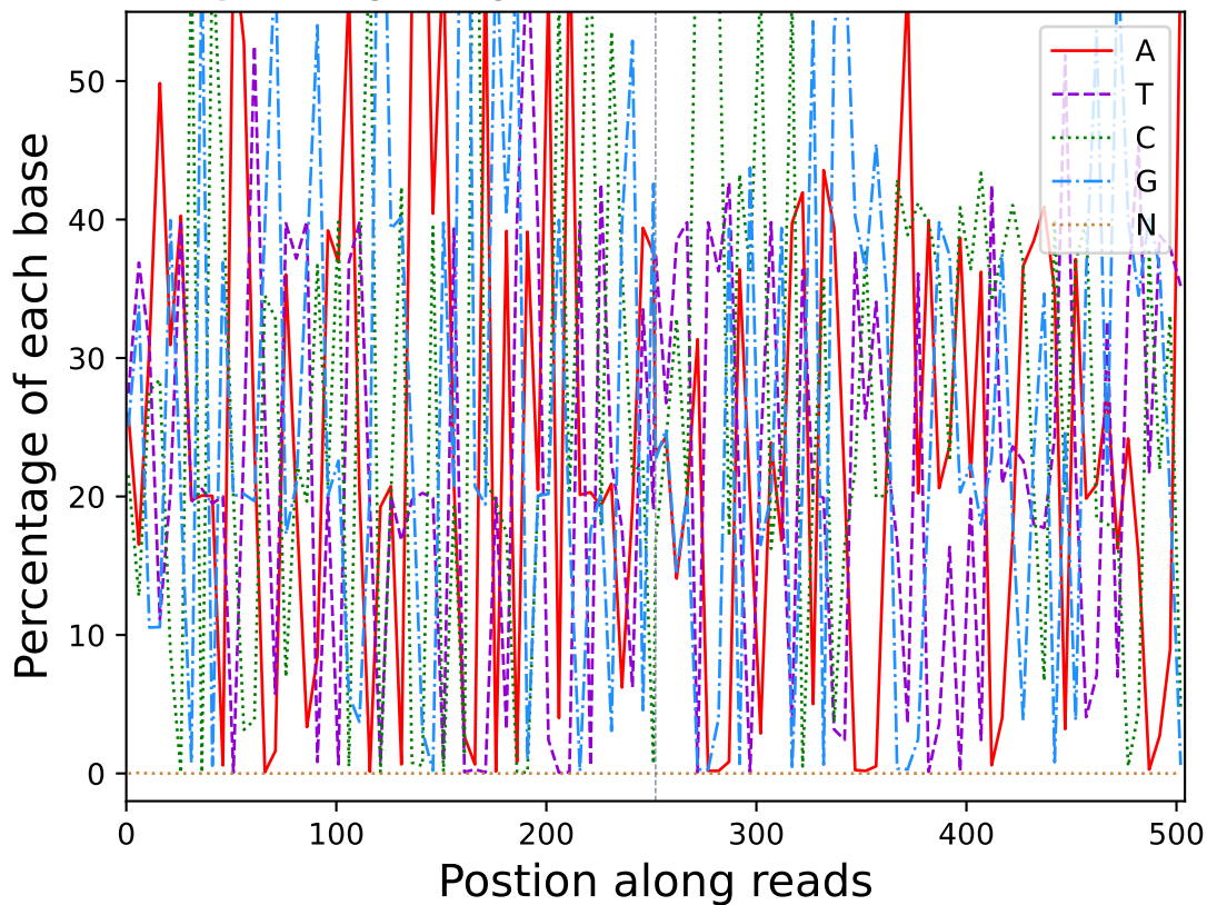
Base percentage along reads (R10316)
